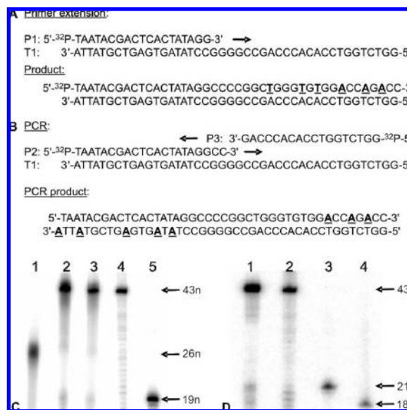
Figure 2. (A and C) Enzymatic incorporation of LNA-T and LNA-A nucleotides using 90 N m DNA polymerase: P1, primer (19n); T1, template (43n). (Lane 1) Negative control reaction with only two natural nucleotides (dCTP and dGTP) present (26n); (lane 2) incorporation of LNA-T and LNA-A nucleotides (43n); (lane 3) positive control using all four natural deoxynucleotides (43n); (lane 4) 43n marker DNA; (lane 5) primer (19n). (B and D) PCR experiments with LNA-A nucleoside 5'-triphosphate: P2, forward primer (21n); P3, reverse primer (18n); T1, template (43n). (Lane 1) dATP was replaced with LNA-ATP; (lane 2) 43n marker DNA strand; (lane 3) forward primer (21n); (lane 4) reverse primer (18n). LNA incorporations are marked in bold and underlined in all product sequences.
