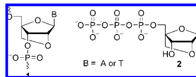
Figure 1. Structural representation of an LNA monomer 1 and LNA nucleoside 5'-triphosphates 2 .
